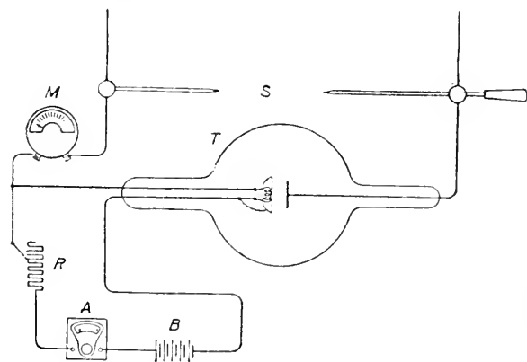
FIG. 35.—Diagram of connections for Coolidge tube.
